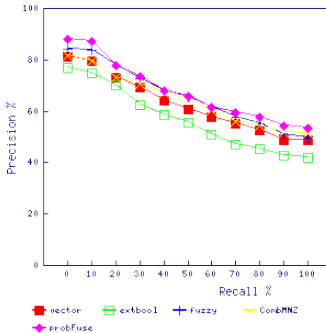
Figure 4. Interpolated Precision graph for the Cranfield collection
