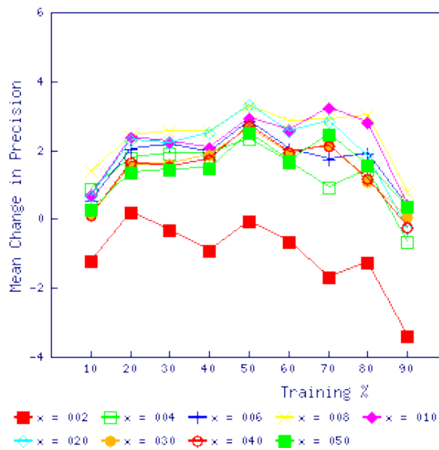
Figure 3. Mean difference in precision for different values of x
